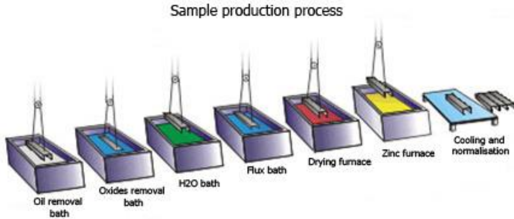
Fig. 1. Schematic representation of experimental setup used for sample production
