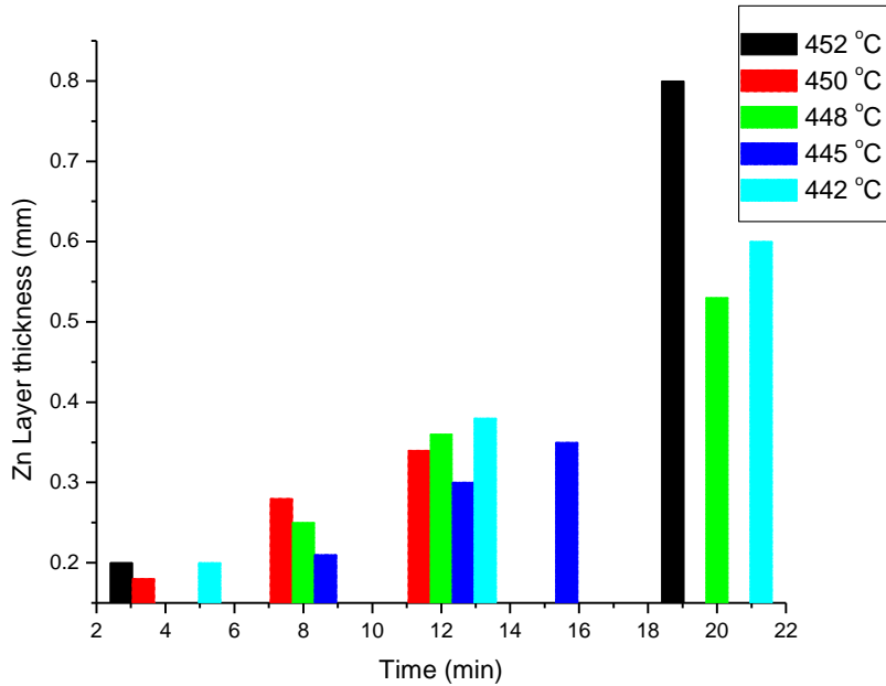
Fig. 4. Zn Layer thickness for different treatment times and temperatures
