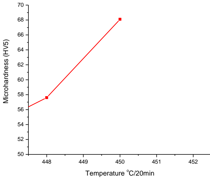
Fig. 2. Microhardness in function of temperature for equal treatment time
