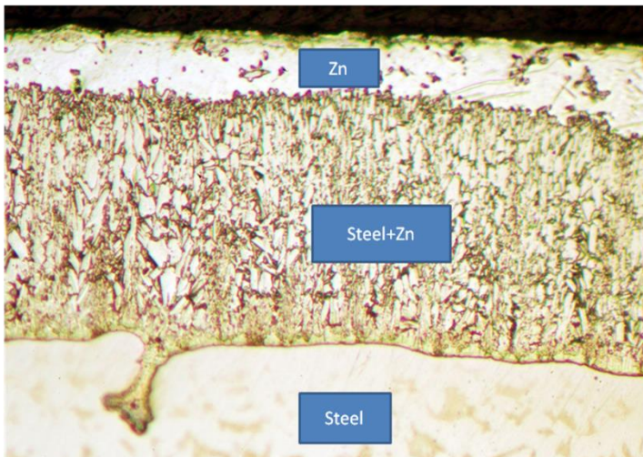
Fig. 3. Optical Microscopy micrograph of cross section of the sample
